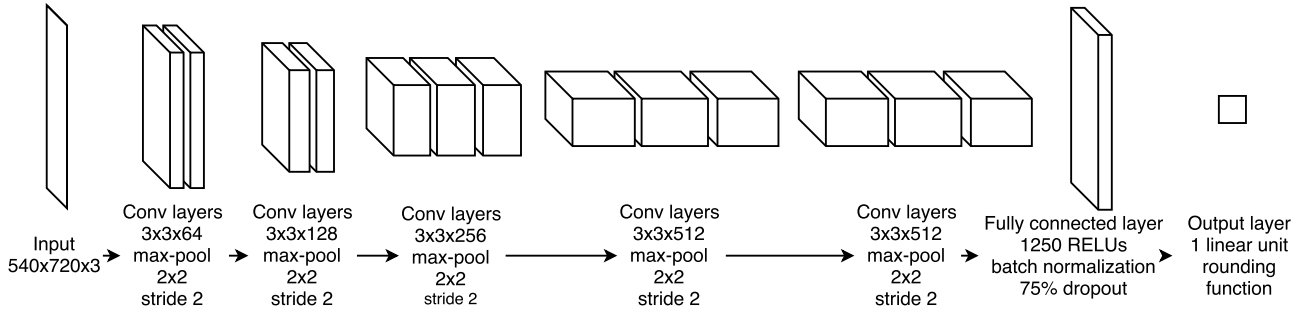
Fig. 2. VGG-16 + regression network architecture.
